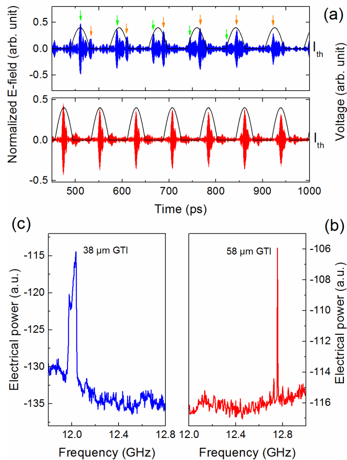
Figure 6: Active mode locked emission as a function of the GTI cavity size. (a) Electric field as a function of time for GTI length of 58 \mu\text{m} (bottom red) and 38 \mu\text{m} (top blue curve). The corresponding active GHz modulation (black lines) are superimposed to the QCL E-field emission. The dephasing as a function of the THz round trip cavity between the THz pulses with respect to the active modulation for the 38 \mu\text{m} GTI is indicated with the green and the orange arrows. (b), (c) show the free running beat note close to laser threshold ( \sim 0.7 \text{ kA}\cdot\text{cm}^{-2} ) for the QCLs with 58 \mu\text{m} and 38 \mu\text{m} GTIs, respectively.
