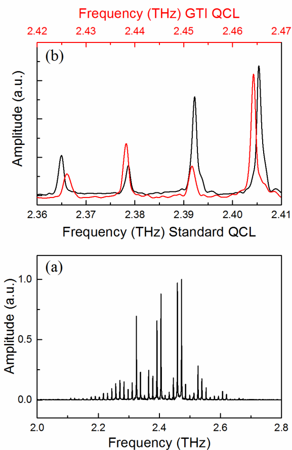
Figure 3: Free running spectral characteristics. (a) Laser spectra of the 2.5 THz QCL (standard) in a metal-metal geometry. (b) Enhance view of Fabry-Pérot modes with a GTI (58 \mu\text{m} length, red line) and a standard cavity (black line).
