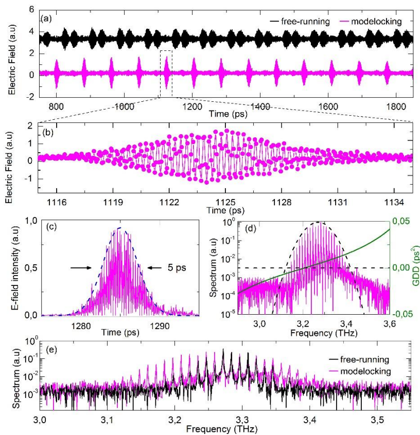
Figure 7: Short pulse generation from dispersion compensated 3.25 THz QCL. (a) The E-field as a function of time for the free running and active modelocked QCL with a 19.5 \mu\text{m} length GTI. (b) Enhanced view of one pulse. Dots corresponds to the time resolution (c) Intensity time profile of one pulse with the pulse duration ( \sim 5\text{ps} ) calculated from a Gaussian fit (blue line). (d) The active mode-locked intensity spectrum (FT of (a)) spanning the range from 3.1 to 3.4 THz. The green curve is the calculated GDD of the GTI with a zero-point crossing around 3.2 THz. (e) The amplitude QCL spectrum in free-running and active modulation conditions.
