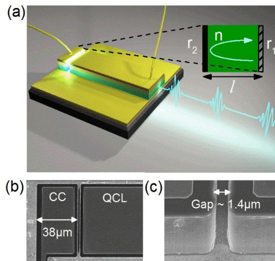
Figure 1. GTI schematic a) Schematic of the GTI coupled to a QCL to realise ultrashort THz pulses. The inset represents the GTI with asymmetric reflectivities, r_1 and r_2 and a cavity length, l . b) SEM image of GTI coupled to QCL cavity c) SEM image of gap between the GTI and the QCL.
