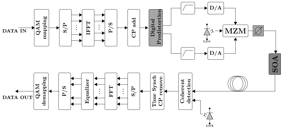
Fig. 1. CO-OFDM structure
