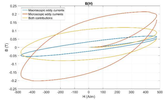
Fig. 1. Hysteresis loop considering different losses contribution.
