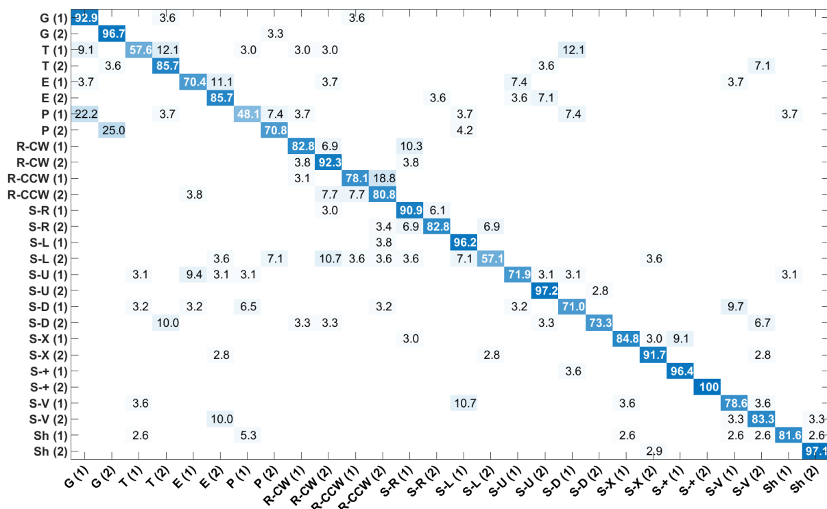
Figure 7: Confusion matrix (28 gesture classes) obtained by De Smedt et al. [DSWV16].
