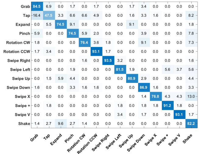
Figure 6: Confusion matrix (14 gesture classes) obtained by Guerry et al.
