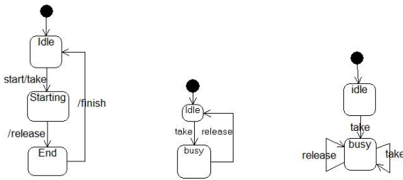
(a) SpecUser (b) SpecResource (c) Resource
