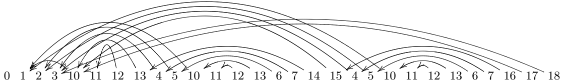
Figure 3: A run of a 2-CPDA
