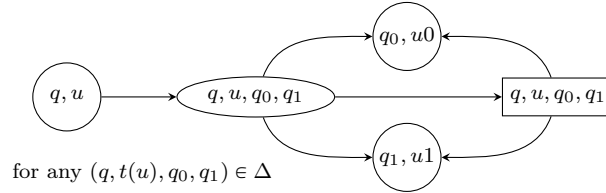
Figure 8: Local structure of the arena of the acceptance game \mathbb{G}_{\mathcal{A},t}^{\text{Acc Uncount}} .
