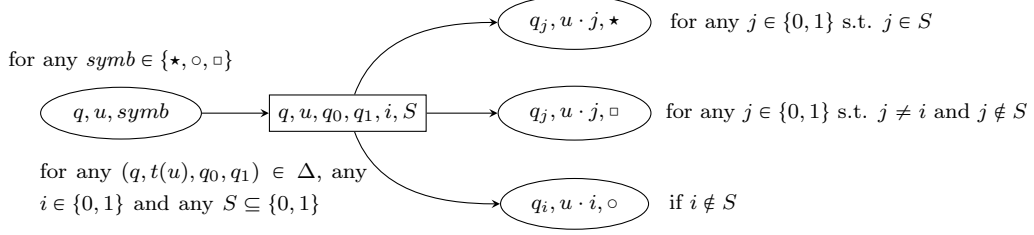
Figure 10: Local structure of the arena of the acceptance game \mathbb{G}_{\mathcal{A},t}^{\text{Acc Large}} .
