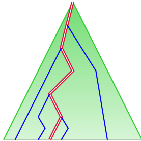
Figure 4: A pseudo comb (U, V)
