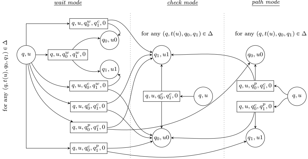
Figure 3: Local structure of the arena of the acceptance game \mathbb{G}_{\mathcal{A},t}^{\text{RejFin}} . We use superscripts to indicate which modes have been proposed by Éloïse.
