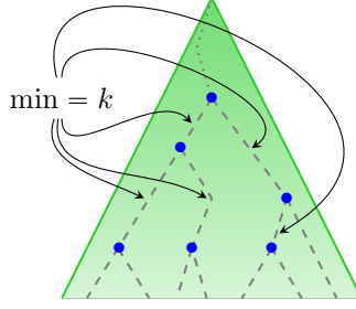
Figure 7: A k -pseudo binary tree U : nodes in U are marked by symbol \bullet .
