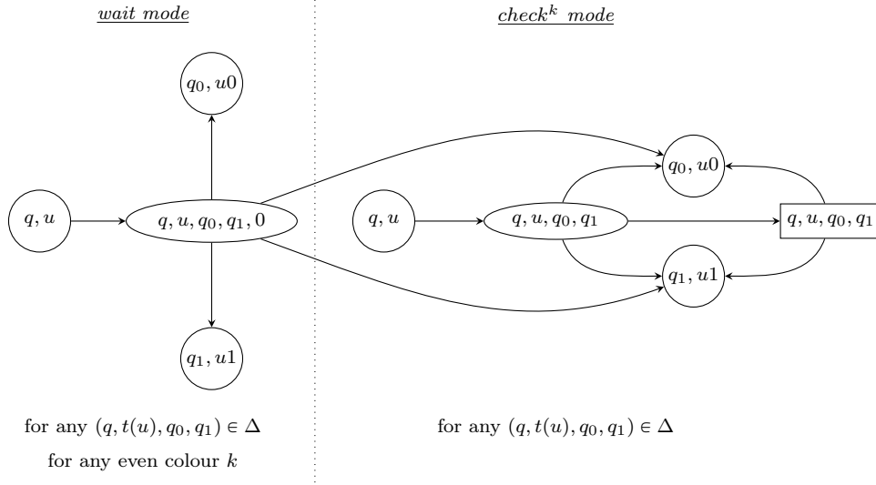
Figure 9: Local structure of the arena of the acceptance game \tilde{\mathbb{G}}_{\mathcal{A},t}^{\text{Acc Uncount}} .
