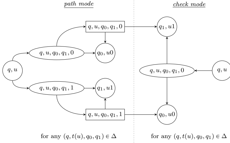
Figure 5: Local structure of the arena of the acceptance game \mathbb{G}_{\mathcal{A},t}^{\text{Acc } \infty} .
