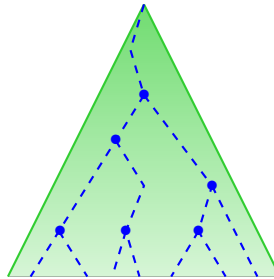
Figure 6: An accepting-pseudo binary tree U : nodes in U are marked by the symbol \bullet and all blue branches are accepting.
