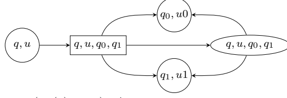
Figure 2: Local structure of \mathbb{G}_{\mathcal{A},t}^{\text{Rej} \leq \text{Count}} .
