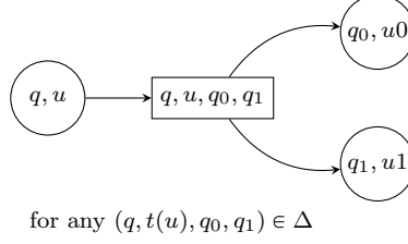
Figure 1: Local structure of the arena of the acceptance game \mathbb{G}_{\mathcal{A},t} .
