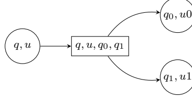
Figure 1: Local structure of the arena of the acceptance game \mathbb{G}_{\mathcal{A},t} .
