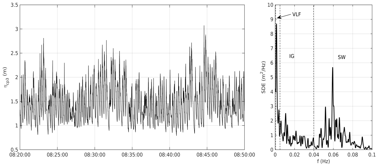
Figure 5. May, 22 swell event, CP3 reef top measurements. Left: free surface elevation from pressure measurements. Right: spectral density of energy.
