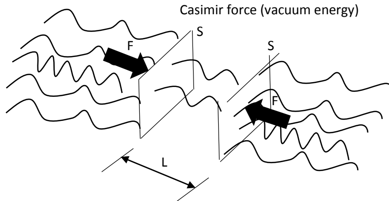
Figure 2 – Definition of the Casimir force confirmed experimentally –
