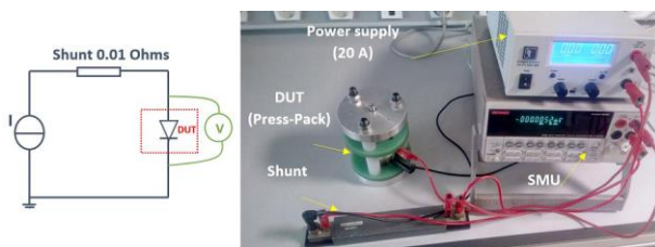
Fig. 7. Picture of the current passage test using 4-point probes method.
