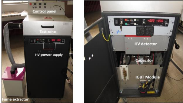
Fig. 6. Picture of the experimental setup using the power circuit in Fig. 3. [7]
