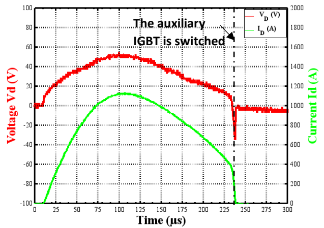
Fig. 8. Voltage and currents waveforms of sample (silver) recorded during the short circuit test @ Tc=25°C.
