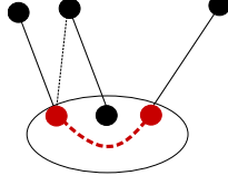
Figure 18: Case (w_i, x_i) = (u_{2i-4}, u_{2i-3}) , y_i = u_{2i} .
