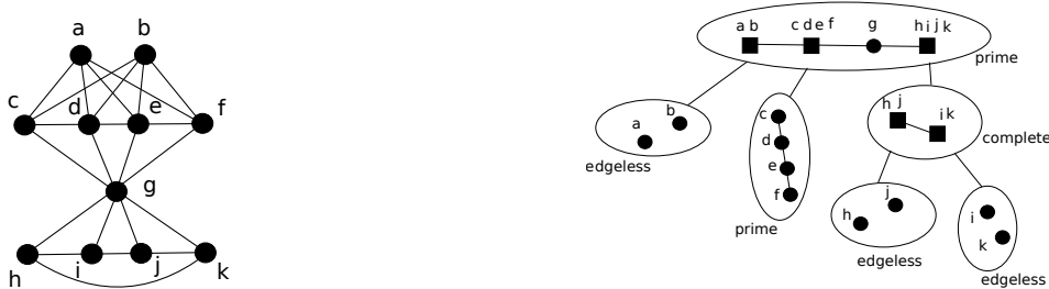
Figure 2: A graph and its modular decomposition.
