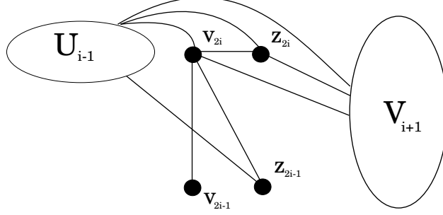
Figure 21: Schematic view of graph G_i .
