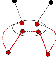
Figure 15: Case x_i, y_i \notin \mathcal{S}_P .
