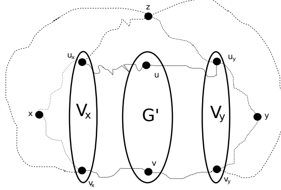
Figure 7: The graph H from the reduction of Theorem 7.
