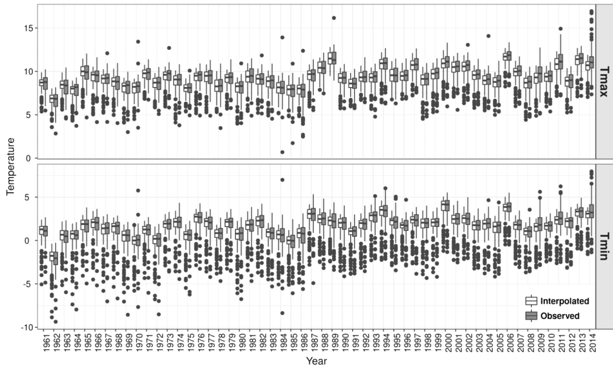
Fig. 3. Inter-annual boxplot of the October to March average minimal and maximal temperature in Burgundy-Franche-Comté for observed (station scale) and interpolated i (grid-scale) data. Each dot is the average T_{\min} or T_{\max} temperature of a station (observed) or its nearest grid point (interpolated). The dark bold line in the boxplot is the median. The two ‘hinges’ of the box are the first (Q1) and third quartile (Q3). The upper whisker is equal to: \min(\max(x), Q3 + 1.5 \times \text{IQR}) ; the lower whisker is equal to: \max(\min(x), Q1 - 1.5 \times \text{IQR}) where IQR is the inter quartile range equal to: Q3 - Q1 , i.e. the box length. A point corresponds to an outlier which is defined as a data point that is located outside the fences (“whiskers”) of the boxplot ( e.g. outside 1.5 times the IQR range above the upper quartile and below the lower quartile).
