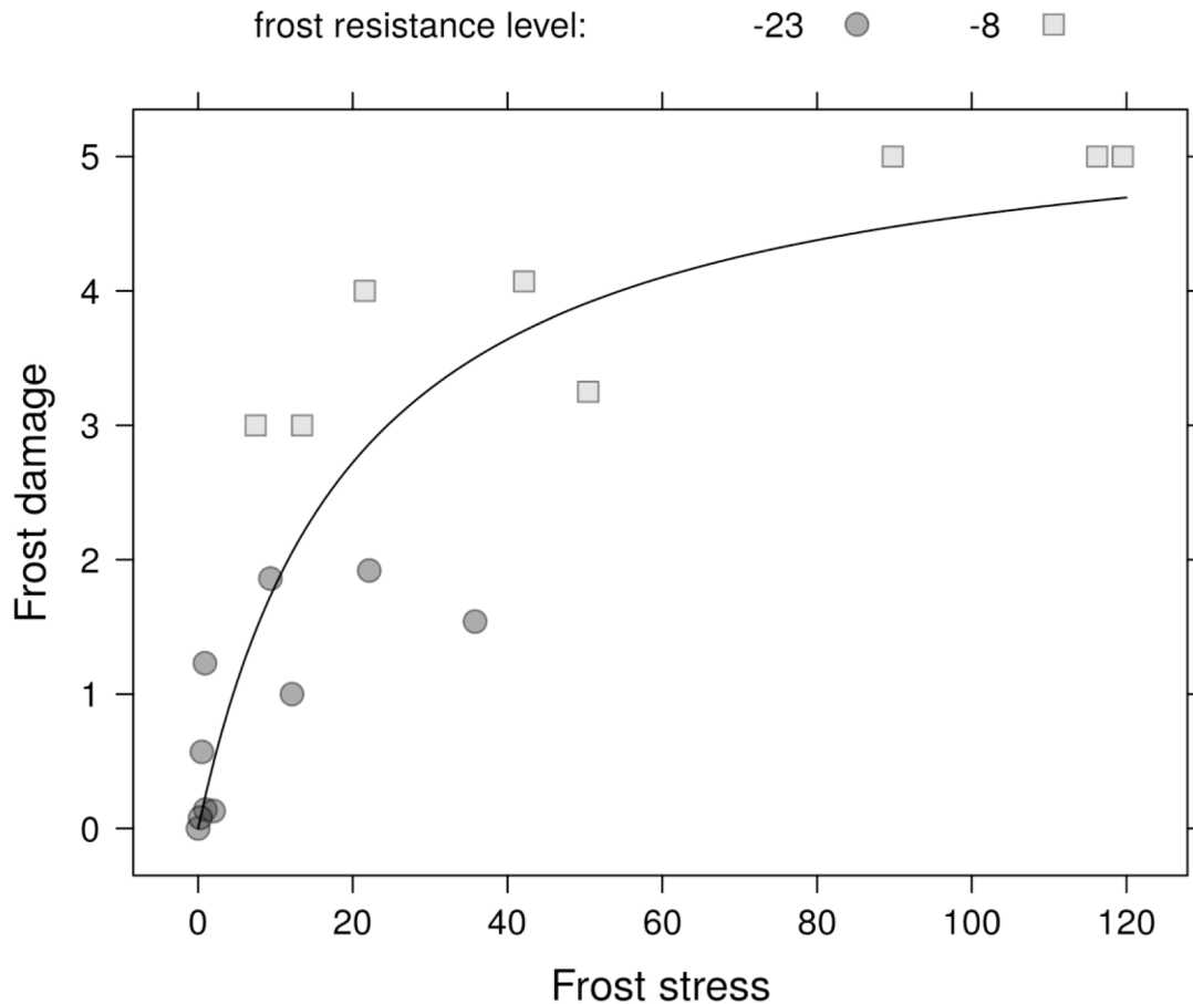
Fig. 4. Cumulative sum of the degree-day of frost stress vs. observed levels of frost damages for two varieties of pea (Champagne and T r se). Frost damages are recorded over 13 experimental trials. The equation of the fitted model is: Frost damage = a \times \text{Frost stress} / (b + \text{Frost stress}) with a = 5.48 and b = 20.3 . The R^2 of the adjustment is 0.76.
