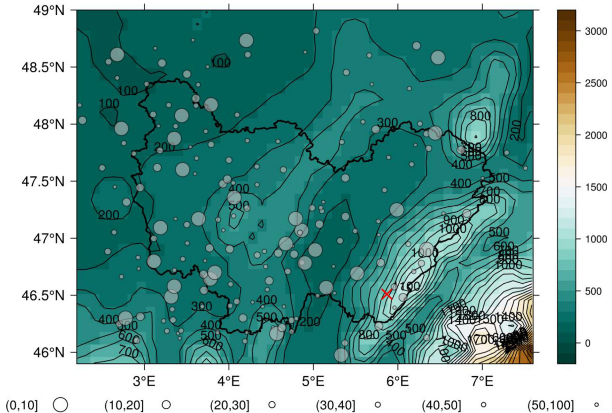
Fig. 2. Relief map of the Burgundy-Franche-Comté region (BLACK bold line) and location of the Météo-France climate stations (grey circles) used for both daily spatial interpolation of temperatures and computation of frost stress level. Note that the circle size is reversely proportional to the missing data in the climate series. Red cross corresponds to the pea crop experimental site located at Chaux-des-Prés. Altitude is given in metres above sea level. Elevated areas in the South-East of the map correspond to the Alps mountains.
