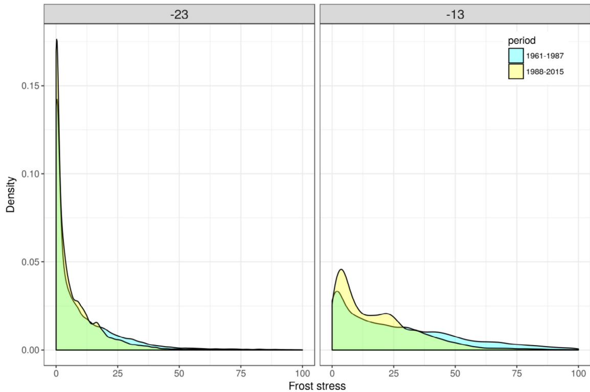
Fig. 6. Frost stress distribution before and after the 1987/1988 temperature shift and for the two stress resistance traits -13^{\circ}\text{C} and -23^{\circ}\text{C} and for all dates of sowing, for rates of acclimation. Green area corresponds to the common area of the two distributions. Cyan color indicates higher probability that frost stress index occurs during period 1961–1987 while for the yellow color it is the reverse. As the frost stress distributions are zero-inflated and left heavy-tailed, a robust Bayesian estimation following the method described in Kruschke (2013) is used to test the difference. The 95% Highest Density Interval (HDI) is a useful summary of where the bulk of the most credible values falls. When the difference is significant means that the 95% HDI interval does not include zero (no difference between periods).
