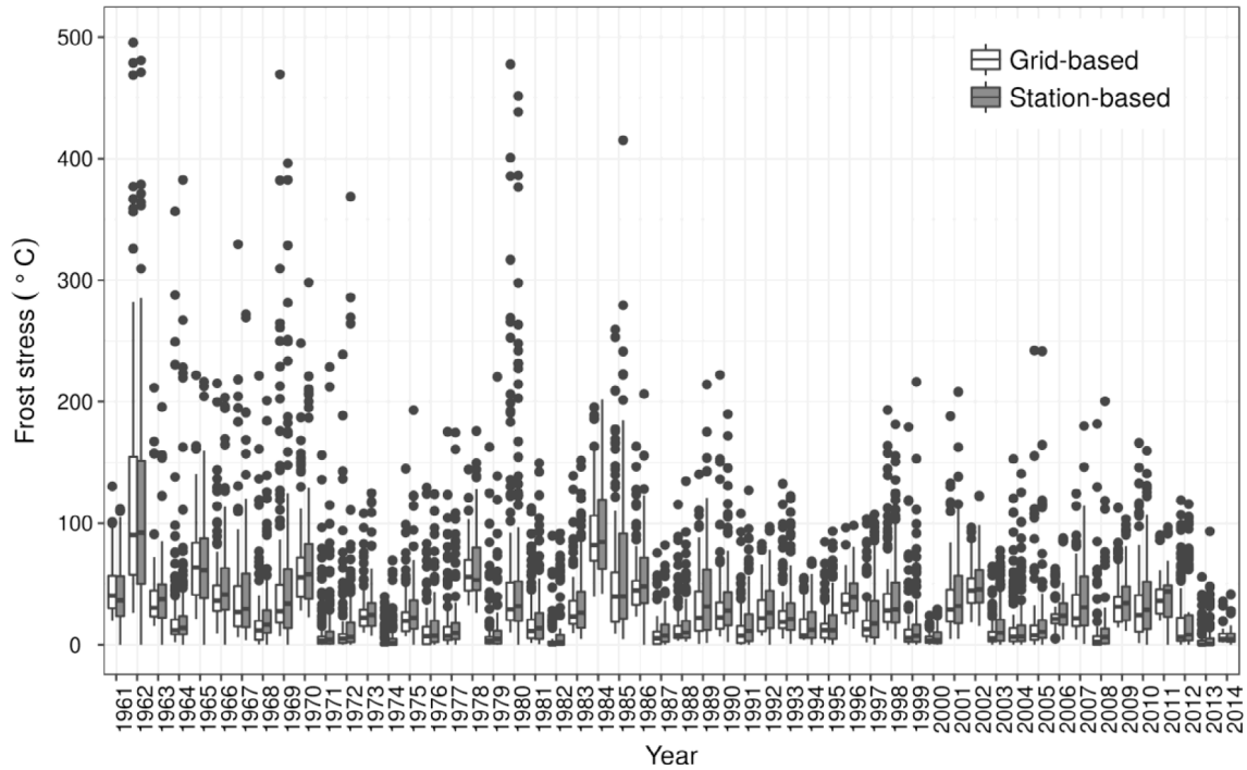
Fig. 5. Boxplot of the inter-annual frost stress index computed from observed (station) and interpolated (grid) climate data. The index is expressed as the cumulative sum of the degree-day of frost stress. The simulations concern the winter pea variety with a frost level resistance of -13^{\circ}\text{C} . A point corresponds to the results of one station (grid), one date of sowing and one rate of acclimation.
