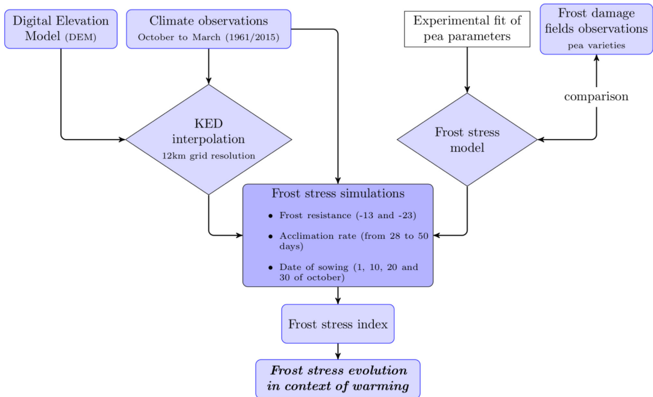
Fig. 1. Flow chart providing an overview of the methodological steps implemented in the framework of this study. The chart consists of two interrelated sections, pointing out for (right) parametrization and assessment of the frost stress model for winter pea crop and (left) daily climate data interpolation at 12-km-grid resolution from 1961 to 2015. KED is the kriging with external drift method which is similar to regression kriging (Hengl et al. , 2007). An automated interpolation based on the AUTOMAP R packages (R Core Team, 2016; Hiemstra et al. , 2009) has been used in this study.
