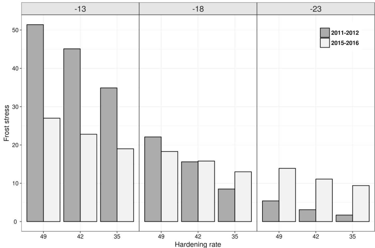
Fig. 7. Simulated frost stress index as a function of both frost resistance ( -13^{\circ}\text{C} , -18^{\circ}\text{C} and -23^{\circ}\text{C} ) levels and acclimation rates (35, 42 and 49 days) for 2011–2012 and 2015–2016 winters. The computation is conducted for Dijon place. The winter T_{\min} and T_{\max} showed contrasted fluctuations during January and February 2012 with an intense cold period of three consecutive weeks (observed minimal T_{\min} of -15.7^{\circ}\text{C} the 5 th of February) subsequent to a relative long warm period. Winter 2015–2016 experimented a minimal T_{\min} of -9^{\circ}\text{C} the 24 th of November 2015 with less fluctuations than winter 2011–2012. Note that the date of sowing is fixed the 25 th of October.
