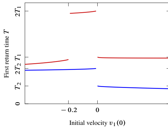
Figure 3: First return time T in the vicinity of LGM: FRT for v_1(0) \approx v_1^{\text{LGM}_1}(0) = 0 of the first LGM [red curves]; FRT for v_1(0) \approx v_1^{\text{LGM}_2}(0) = 0 of the second LGM [blue curves].
