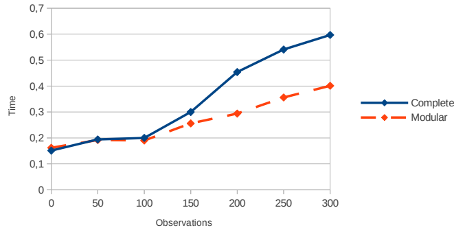
Fig. 5. Average reasoning time of a rabbit regarding the quantity of observations: the dot line correspond to reasoning with decision modules and the plain line without.
