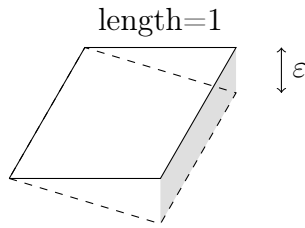
FIGURE 7. Comparing the area of the two parallelograms
