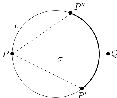
FIGURE 1. Illustration of Lemma 3.1
