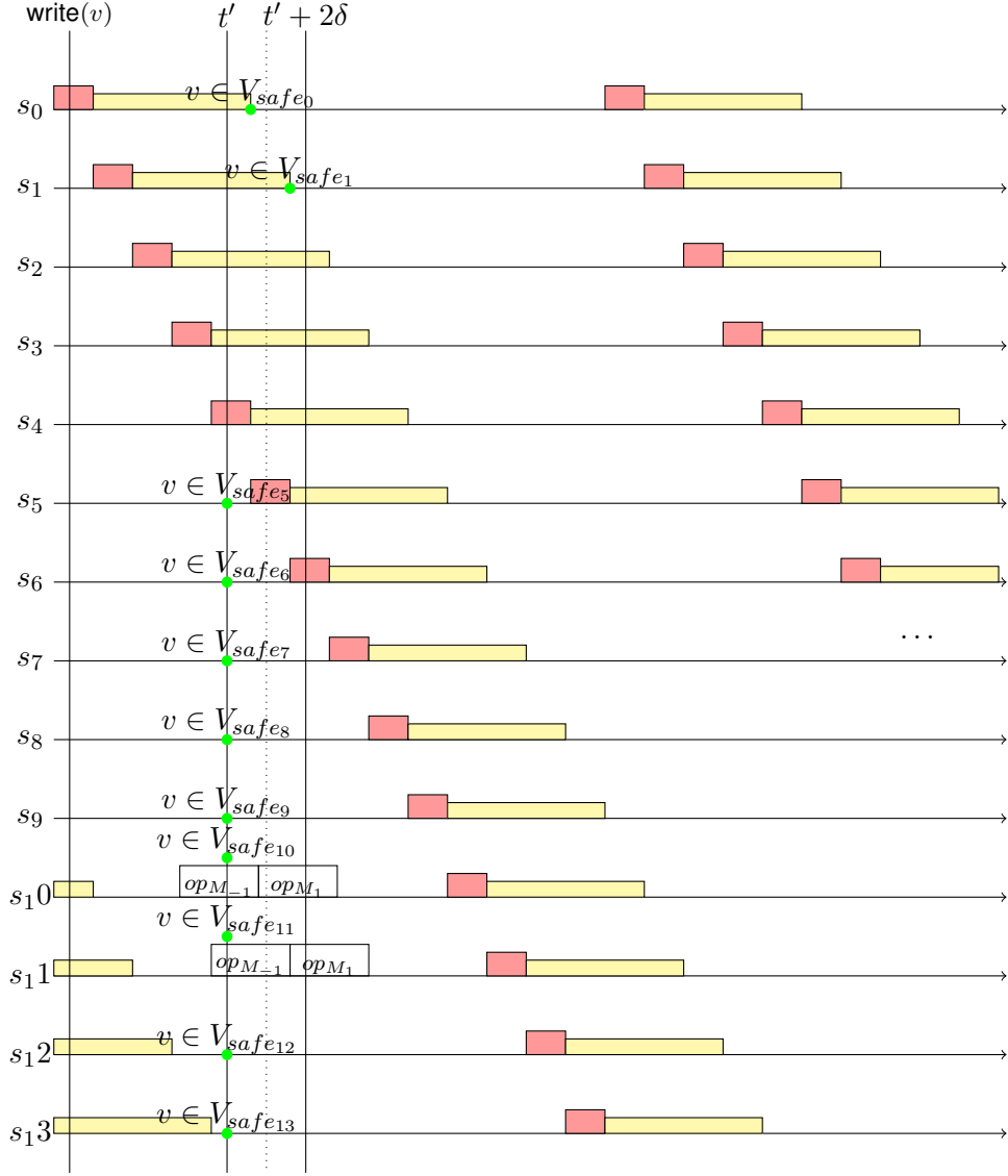
Figure 14: \text{maintenance}() operation op_{M_1} analysis after a \text{write}() operation, t' = t + 4\delta . White rectangles are \text{maintenance}() operation run by correct servers. In particular s_{10} runs such operation during the first \delta period after t' , while s_{11} runs it during the second \delta period.
