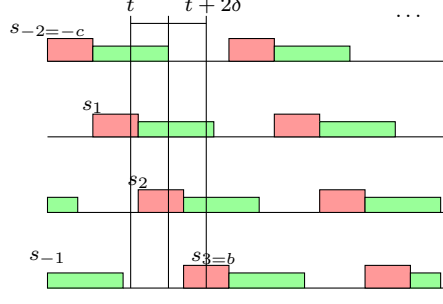
Figure 6: Representation of S^* when we consider a (\Delta S, CAM) model, in particular t_E B(s_1) = t + \epsilon , for \epsilon > 0 and arbitrarily small.
