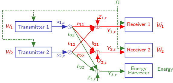
Fig. 1. Two-user Gaussian interference channel with a non-located energy harvester.
