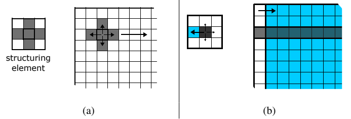
Fig. 2. Computation of a dilation (a) using a neighbourhood iterator or (b) by line translation.
