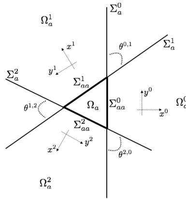
Fig. 8. \Omega_a is a triangle and some associated notations
