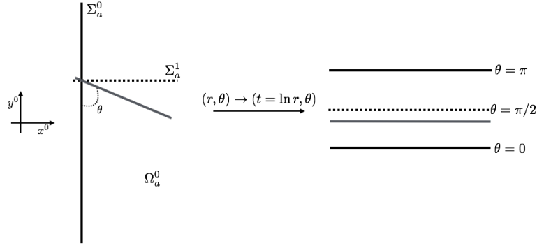
Fig. 5. Notations and change of variable
