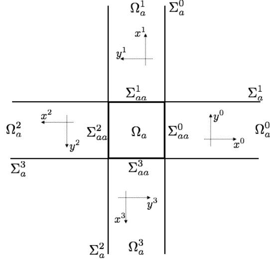
Fig. 1. The notations defined in (2.2-2.3-2.4).
