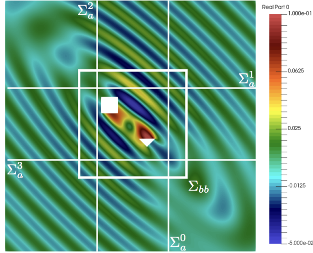
Fig. 4. Real part of the computed solution in \Omega_b and reconstruction of the solution in the halfspace \Omega_a^j .
