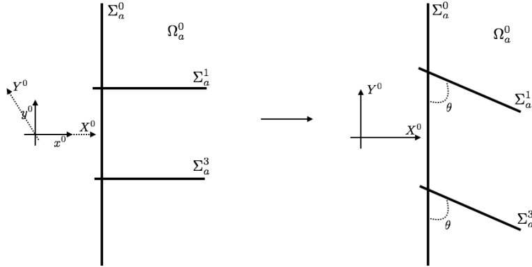
Fig. 6. Change of variable (x_0, y_0) \rightarrow (X_0, Y_0)
