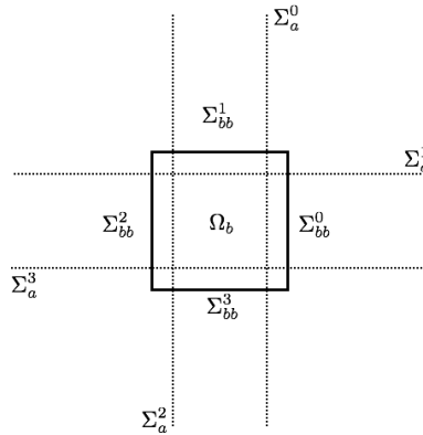
Fig. 2. Second set of notations (2.19) (with the dashed lines are the \Sigma_a^j 's defined in (2.3)).
