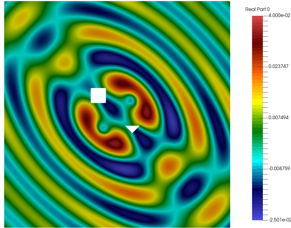
Fig. 7. The solution in an anisotropic non dissipative case with \omega = 10
