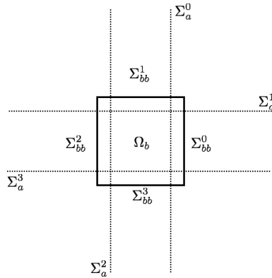
Fig. 2. Second set of notations (2.19) (with the dashed lines are the \Sigma_a^j 's defined in (2.3)).
