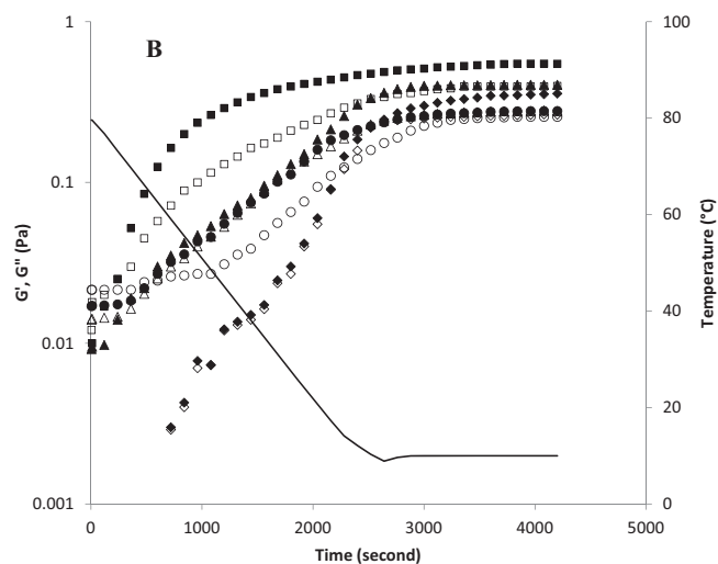
Fig. 4. Semi-logarithmic plots of G' and G'' vs time obtained at constant frequency (1 Hz) during controlled cooling ( 2^\circ\text{C}/\text{min} ) of pectin gels at pH3 (A) and pH 7 (B). G' Ac: (◆), G'' Ac: (◇), G' Ga: (▲), G'' Ga: (△), G' Ne: (●), G'' Ne: (○), G' To: (■), G'' To: (□), Temperature: (-).
