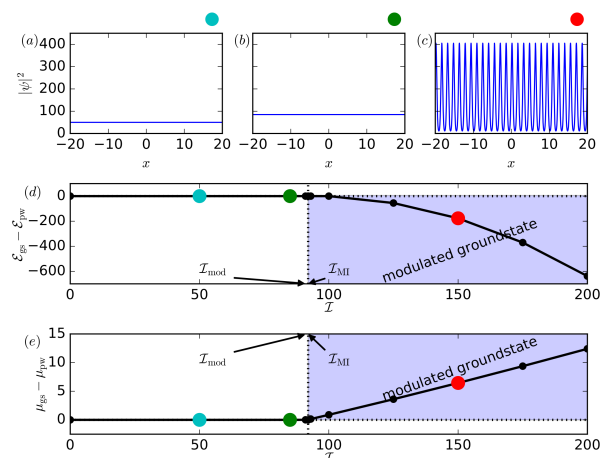
Figure 3: (colour online) (a-c) show ground states for different intensities \mathcal{I} = 50, 85, 150 and \alpha = 1/2, \sigma = 1/2 (compare to Fig. 2). Figure (d) shows the difference of the energy between the numerically exact ground state and the plane wave as function of the intensity. Thus, the intensity \mathcal{I}_{\text{mod}} at which the line \mathcal{E}_{\text{gs}}(\mathcal{I}) - \mathcal{E}_{\text{pw}}(\mathcal{I}) starts to deviate from zero marks the point at which the phase transition from plane wave to modulated ground states occurs. Clearly, \mathcal{I}_{\text{mod}} = \mathcal{I}_{\text{MI}} , and thus the phase transition occurs at vanishing roton gap (see Fig. 2). Figure (e) shows, that the chemical potential \mu does not jump at the point of the phase transition, thus the phase transition is of second order.
