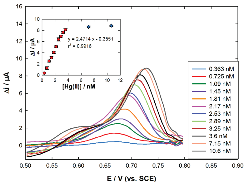
Figure 5. SWASV responses obtained in a 0.01 M HCl solution for increasing Hg(II) concentrations (blank subtracted) on a AuNPs(B)-GC electrode. Inset: \square i_p vs. [Hg(II)] and corresponding linear regression.
