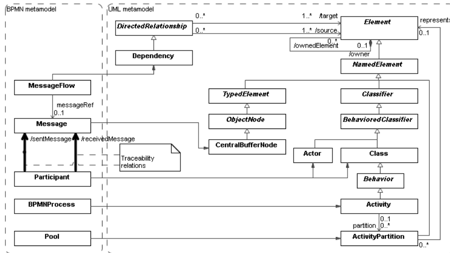
Fig. 8. Parts of BPMN and UML metamodels extended with traceability relation between participants and messages sent or received by the participant
