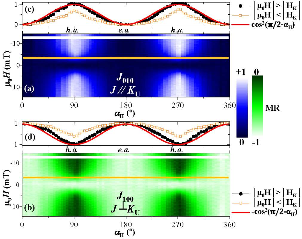
Figure 6. Two-dimensional map representations of the RT angular evolution of the forward branches of the MR curves of LSMO film deposited onto 6^\circ vicinal STO(001). Panel (a) shows the case of current injected along the [010] direction ( J_{010} ), panel (b) the case of current injected along the [100] ( J_{100} ). This graphic representation allows the identification of two-fold (uniaxial) symmetry with 180^\circ periodicity. By cutting the maps horizontally we get an angular evolution of MR at fixed magnetic field. By doing so, at field larger than the anisotropy field [ \mu_0H = -13 mT, black-circles in insets (c,d)] we obtain a good agreement with \cos^2\alpha_H , whereas for smaller field [ \mu_0H = -3.7 mT, orange-squares in insets (c,d)] such a dependence is not valid.
