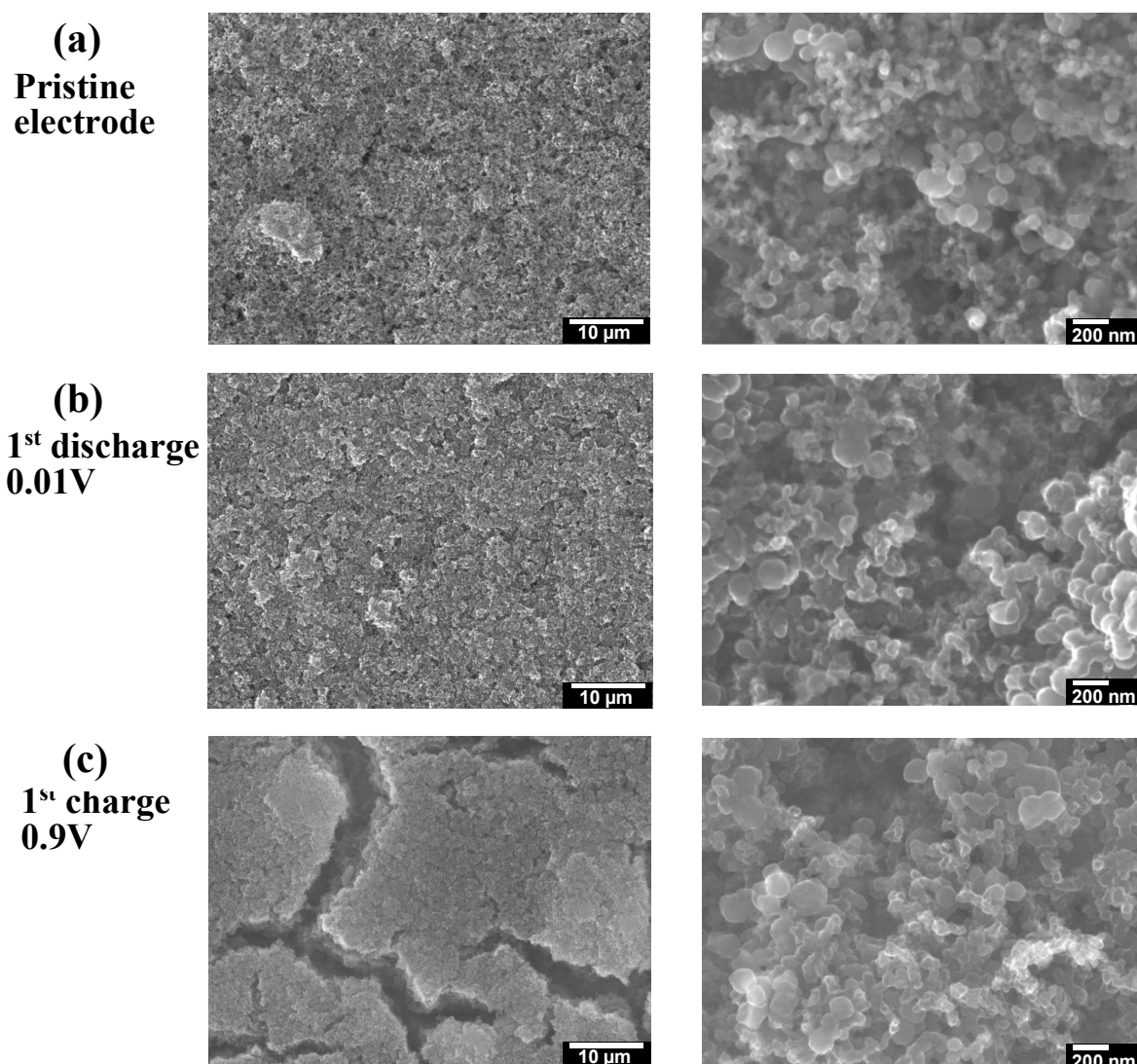
Figure 3: SEM images (10 μm and 200 nm scales, horizontal bars) of the Si/C/CMC composite electrode (a) pristine electrode, (b) after discharge at 0.01 V, (c) after charge at 0.9 V.
