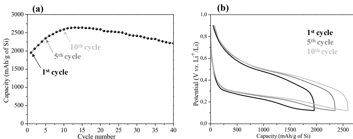
Figure S1: (a) Discharge capacity vs. cycle number of Li//Si cells (cycling between 0.12V and 0.9V with a rate of 150 mA/g of Si) using LiFSI. (b) Potential vs. capacity curves of the 1 st , 5 th and 10 th cycles (Precycling is not shown).
