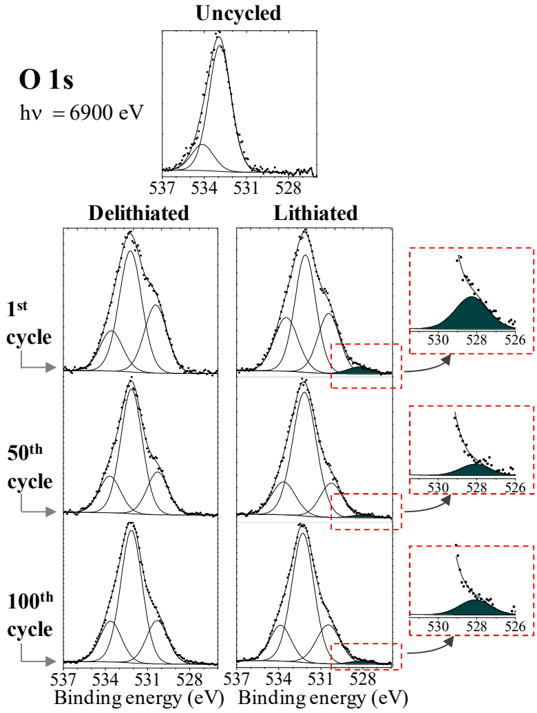
Figure 5: O 1s spectra of the Si electrode soaked 5 days in the electrolyte (uncycled), and after the 1 st , 50 th and 100 th discharges (lithiated) and charges (delithiated) with an electrolyte containing LiFSI. A zoom of the low B.E. region is shown on the right to highlight the signature of Li 2 O. (hv = 6900 eV)
