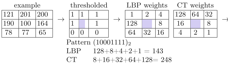
Fig. 1. Neighbors of center pixel g_c participating in LBP or CT code generation in the case of a 3 \times 3 neighborhood ( P = 8 and R = 1 ).
