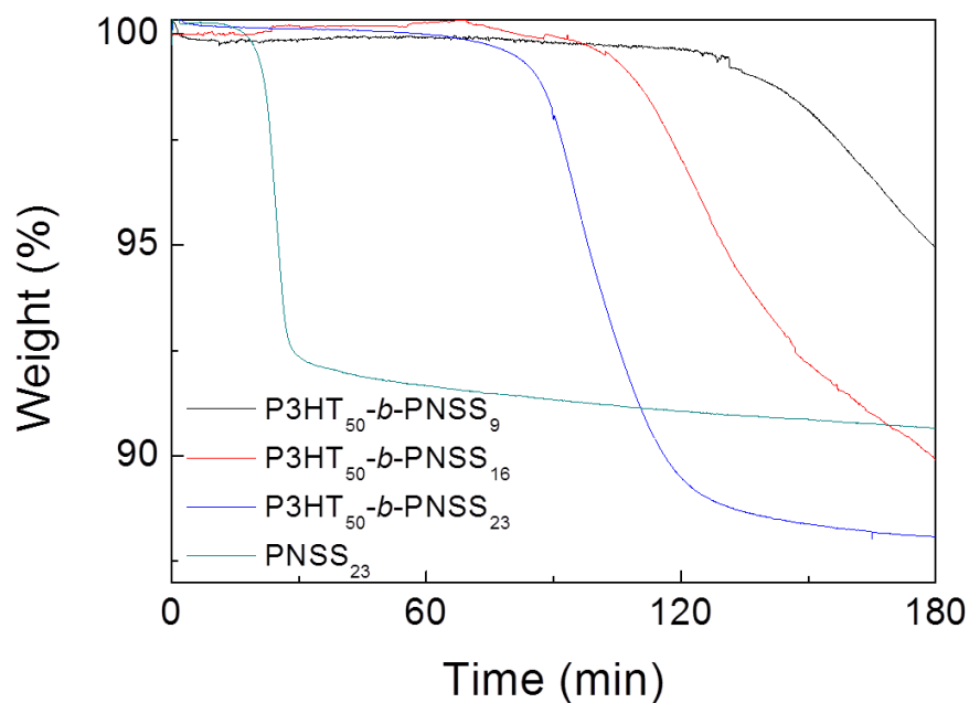
Figure 4. Thermogravimetric isotherms at 150 °C of the three P3HT 50 - b -PNSS x block copolymers alongside PNSS 23 homopolymer as a control.
