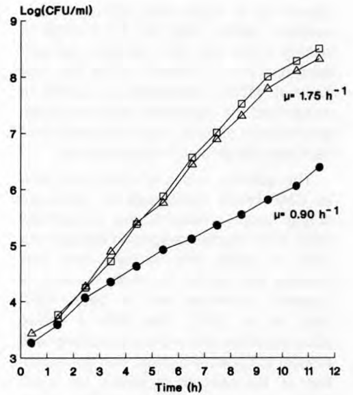
Fig 2. Effects of SP (50 µg/ml) (—□—) and LP (2 mg/ml) (—△—) on L. lactis growth as determined by cells enumeration on M17 medium (—●—) control culture. \mu = growth rate.
