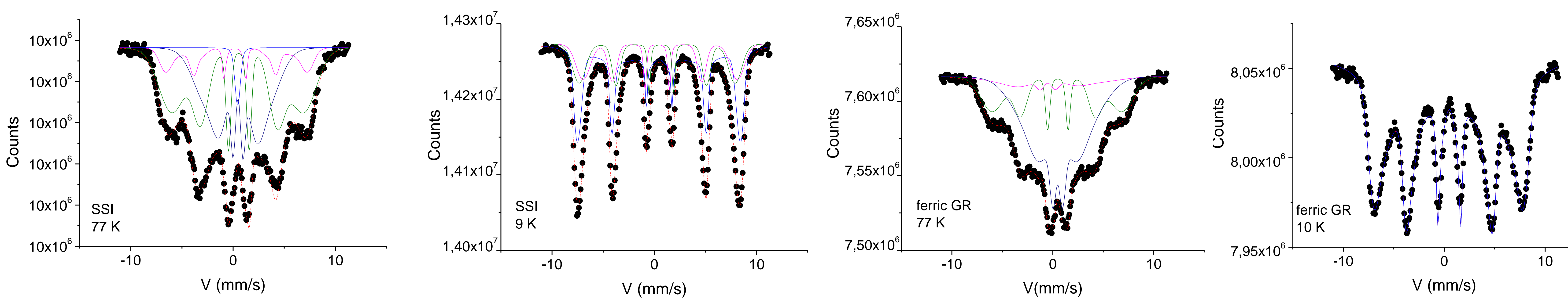
Spectres Mössbauer de SSI
