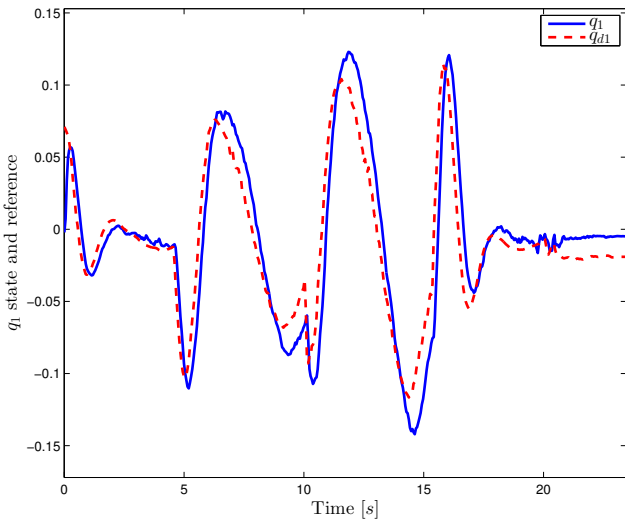
Fig. 37 Attitude and reference for q_1 in case 2 experiments.
