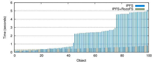
Fig. 2: Reading time of each object for a given client and a given iteration ( 100 \times 256 KB).
