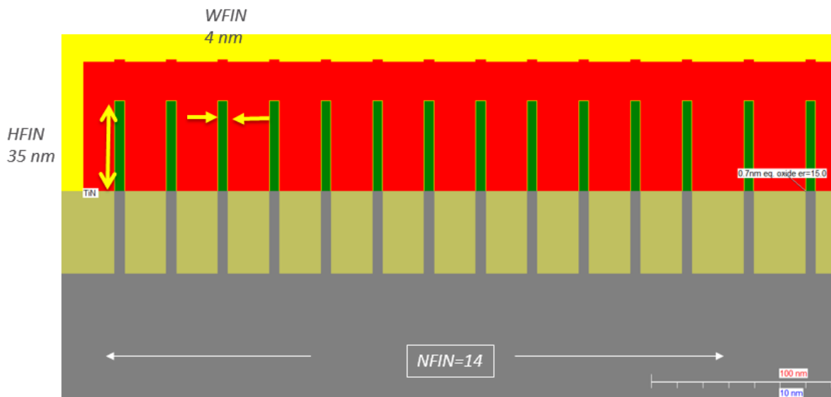
Figure 8: The equivalent width of a multi-fin FET
