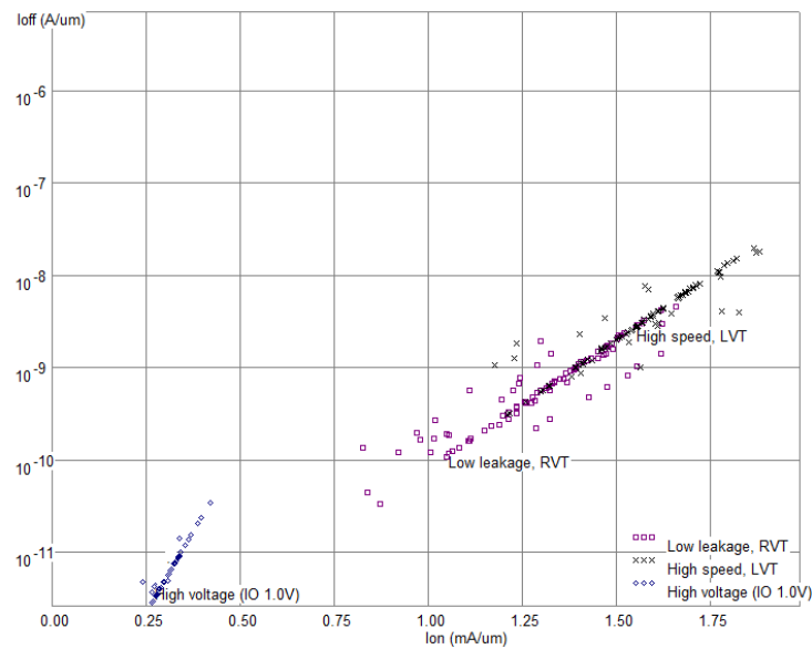
Figure 17: I_{off}/I_{on} calculated on 100 samples of n -FinFET with random distribution of V_T and U_0 , with a Gaussian distribution around the nominal value
