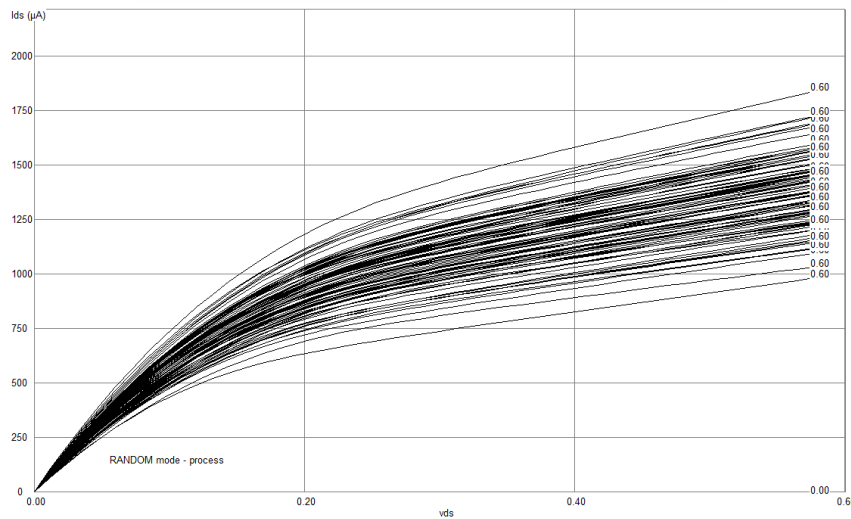
Figure 15: I_{ds} vs V_{ds} calculated on 100 samples of n-FinFET with random distribution of V_T and U_0 , with a Gaussian distribution around the nominal value.
