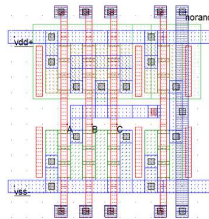
Figure 20: Compilation of a combination of AND and OR cells, with verification of the design rules
