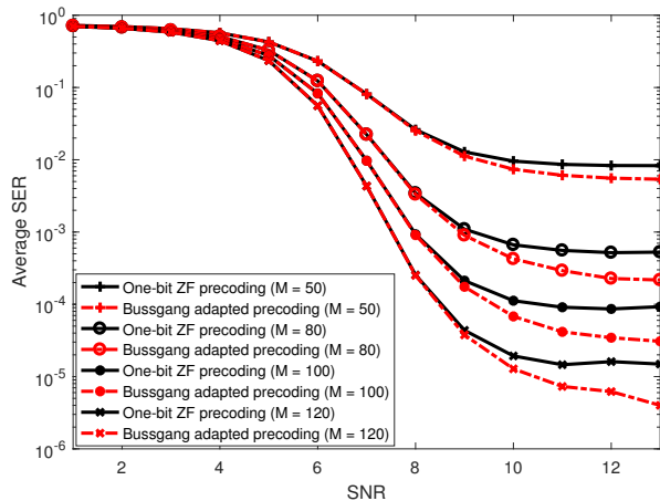
Fig. 9: Variation of SER for one-bit quantized Bussgang adapted and ZF precoding versus SNR for K = 10 users and varying values of M .
