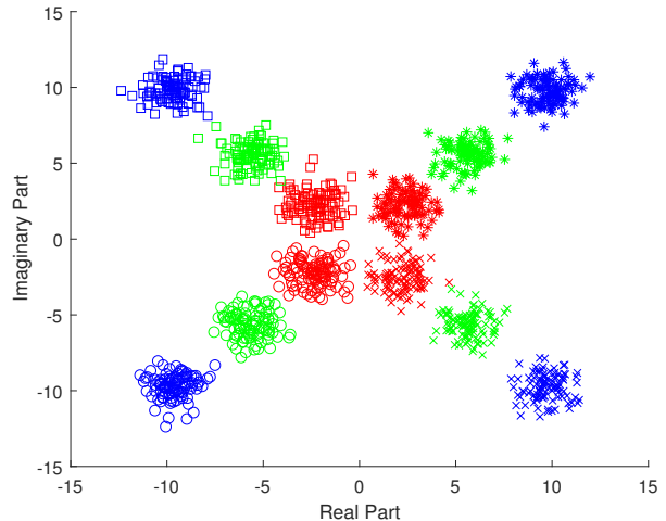
Fig. 7: Plot of the received vector in a noiseless scenario, for K = 4 , and different values of M , M = 20 (red), 100 (green), 300 (blue). Different components of the received vector are shown as different symbols.
