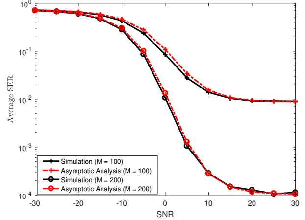
Fig. 5: Variation of SER with SNR for K = 20 users with unequal channel gains and varying values of BS antennas M .
