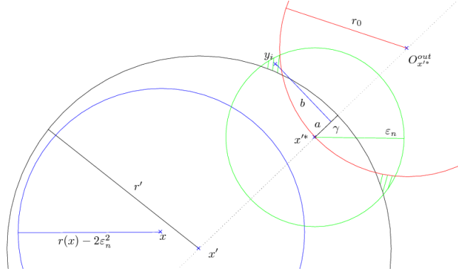
Figure 4: Let B(x', r') \in \mathcal{C}^{\max}(\hat{S}_n, \mathcal{Y}) and x'^* be a point of \partial S such that d(x', \partial S) = \|x' - x'^*\| . Then there exists a y_i \in \mathcal{Y} in the green dashed area.
