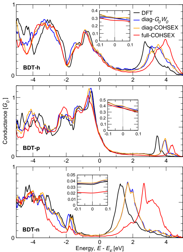
FIG. 2. Conductance \mathcal{G}(E) in units of \mathcal{G}_0 as a function of the energy E for BDT-h (top panel), BDT-p (middle) and BDT-n (bottom panel). Black line: DFT; blue line: diag- G_0W_0 ; yellow line: diag-COHSEX; red line: full-COHSEX. The insets are zooms over the zero-bias conductance \mathcal{G}(E=0) region. The zero of the energy is set to the Fermi energy E_F .
