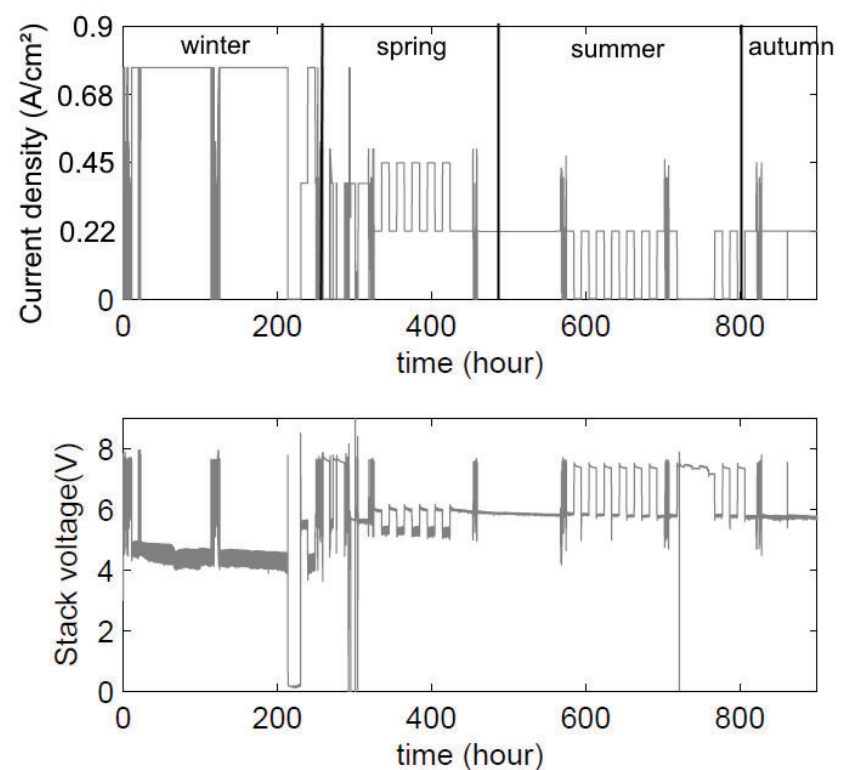
Fig. 2. Load current and recorded stack voltage
