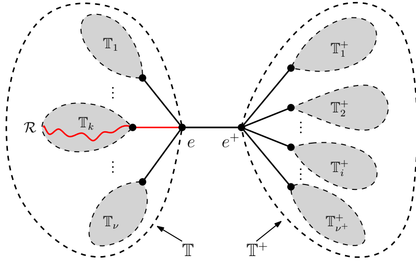
Figure 1: The random tree \mathbb{T}\text{-}\bullet\mathbb{T}^+ rooted at e^+ with a marked ray \mathcal{R}
