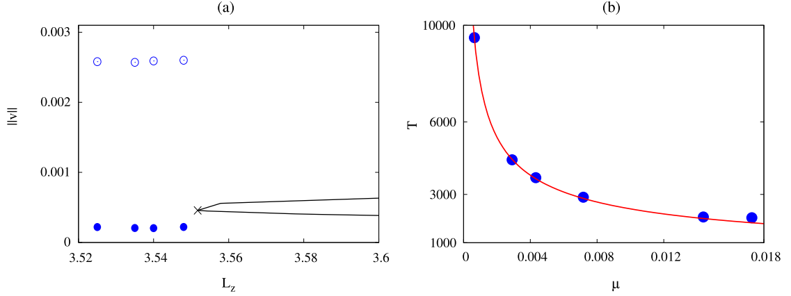
Fig. 2. (a) Bifurcation diagram in L_z , with L_x = 2\pi and Re = 2000 , where the relative periodic orbit solution disappears in a global saddle-node infinite-period bifurcation originating a pair of travelling-wave solutions. The periodic solution is reported with its maximum (empty symbols) and minimum (filled symbols) values of the spatially-averaged wall-normal velocity. The symbols correspond to the L_z values considered in Fig. 1. The point where the upper- and lower-branch travelling-wave solutions are generated is denoted by the X symbol. (b) Variation of time period T close to the bifurcation point. The function T \approx 240/\sqrt{\mu} (solid line), where \mu = (L_z^* - L_z)/L_z^* , fits well the data (symbols). The four leftmost symbols correspond to the time-series reported in Fig. 1.
