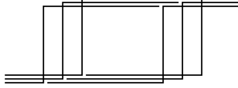
Figure 1: A complete graph K_6 minus a matching.
