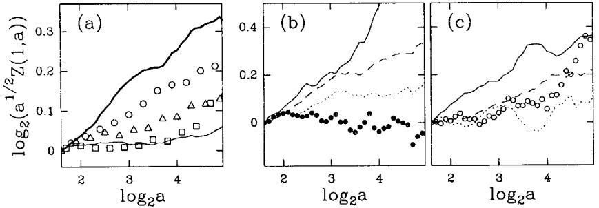
Fig. 4. a^{1/2}Z(q = 1, a) vs. a in logarithmic scales, when averaged over 42 coding and 74 noncoding human DNA sequences. (a) introns (—), CDSs (---), coding subsequences relative to position 1 ( \triangle ), 2 ( \square ) and 3 ( \circ ) of the bases within the codons. (b) Introns: ( \cdots ) GC% = 31.6 \pm 0.4 , L = 15210 ; ( --- ) GC% = 48.6 \pm 1.0 , L = 17137 ; ( --- ) GC% = 63.3 \pm 0.9 , L = 10449 ; ( \bullet ) first intron of the human factor XIIIb subunit gene with GC% = 31.2, L = 2874 . (c) Coding subsequences relative to position 3 of the bases within the codons: ( \cdots ) GC% = 38.1 \pm 2.9 , L = 4759 ; ( --- ) GC% = 50.8 \pm 2.8 , L = 28521 ; ( --- ) GC% = 62.5 \pm 2.1 , L = 16558 ; ( \circ ) exon of the human apoB-100 gene with GC% = 41.0, L = 7571 . The analyzing wavelet is \psi^{(2)} .
