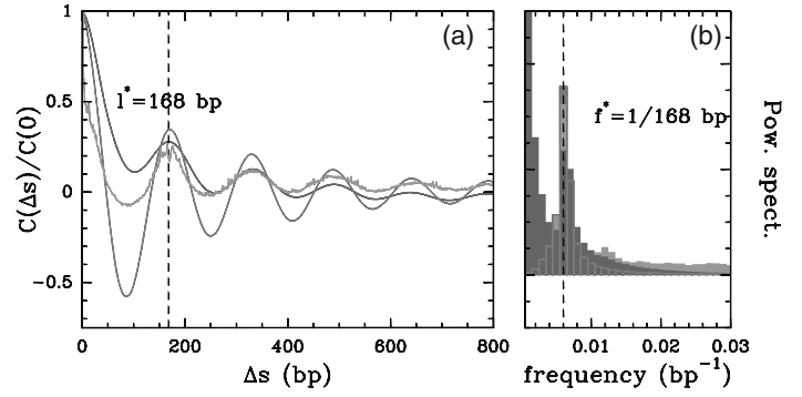
Figure 8. (a) Auto-correlation function C(\Delta s) = \langle \delta Y(s) \delta Y(s + \Delta s) \rangle versus \Delta s . (b) Corresponding power spectrum. The different colors correspond to the following S. cerevisiae data sets: MNase-chip data of Lee et al. (2007) (red) and of Whitehouse et al. (2007) (blue); MNase-seq ‘tag’ data of Shivaswamy et al. (2008) (green).
