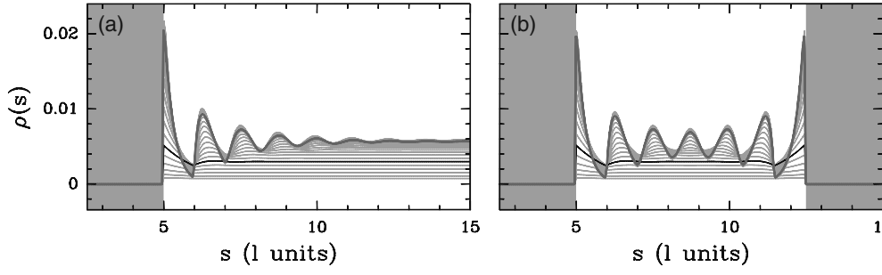
Figure 18. Evolution of the density profile \rho(s) with the chemical potential \tilde{\mu} from \tilde{\mu} = -5 kT (black) to +5 kT (red). Statistical confinement near an infinite wall (a) and in between two infinite energy barriers (b).
