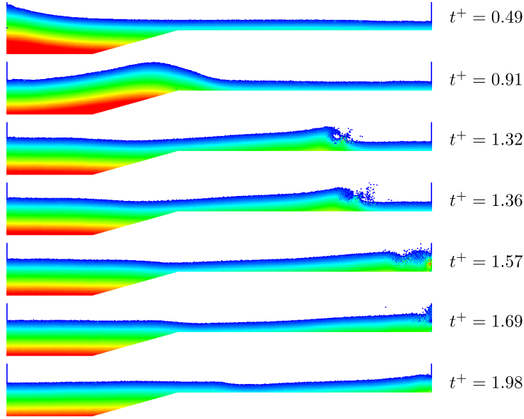
Figure 6: Propagation of a solitary wave on a slope with \nu = 10^{-6}m^2s^{-1} ; pressure field obtained with ISPH-USAW ranging from 0Pa to 5837Pa (blue to red).
