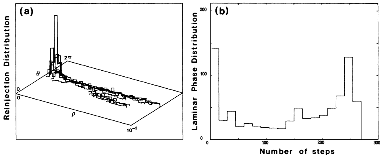
FIG. 4. (a) Reinjection distribution inside the two-dimensional unstable manifold of the fixed point \rho = 0 and (b) probability distribution P(n) for the laminar lengths; same model parameters as in Fig. 1(c).
