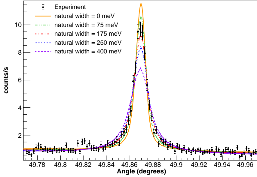
FIG. 10: (Color online) Example of a dispersive-mode experimental spectrum for the Be-like Ar 1s2s^22p^1P_1 \rightarrow 1s^22s^2^1S_0 transition (black dots), together with a few plots of the function in Eq. (1), for different values of the natural line width \Gamma_L^i . The four parameters have been adjusted to minimize the reduced \chi^2(\Gamma_L) (see text for more explanations).
