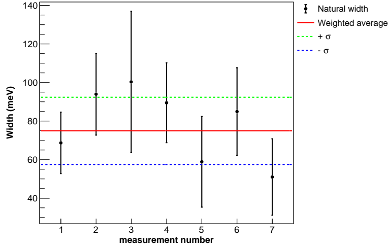
(a) He-like argon 1s2p\ ^1P_1 \rightarrow 1s^2\ ^1S_0 transition.
