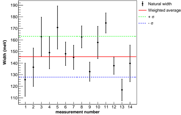
(b) Be-like argon 1s2s^2p\ ^1P_1 \rightarrow 1s^22s^2\ ^1S_0 transition.
