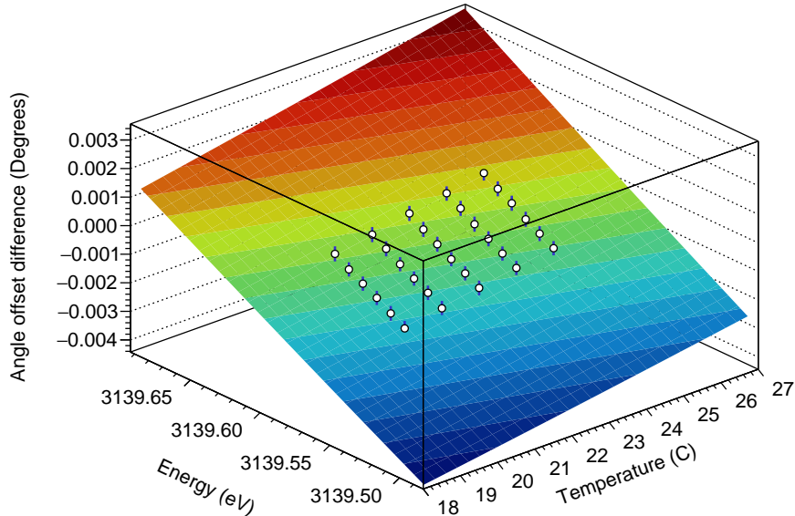
FIG. 4: (Color online) Fitted two-dimensional function from Eq. (4), and experimental results (white spheres), for the He-like Ar 1s2p^1P_1 \rightarrow 1s^2^1S_0 transition. The fit is performed taking into account the statistical error bars in each point.
