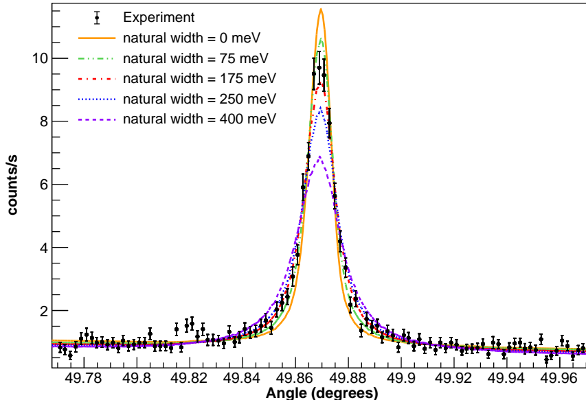
FIG. 10: (Color online) Example of a dispersive-mode experimental spectrum for the Be-like Ar 1s2s^2 2p^1 P_1 \rightarrow 1s^2 2s^2 1 S_0 transition (black dots), together with a few plots of the function in Eq. (1), for different values of the natural line width \Gamma_L^i . The four parameters have been adjusted to minimize the reduced \chi^2 ( \Gamma_L ) (see text for more explanations).
