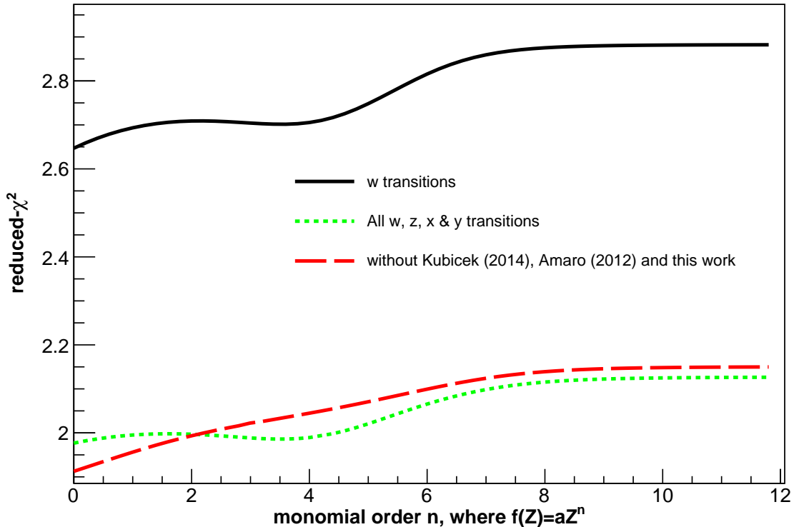
FIG. 7: (Color online) Values of the reduced \chi^2 function as a function of n , when fitting aZ^n , n = 0 to 12 , to the experiment-theory differences from Tables VII and VIII. Solid line: reduced \chi^2 fitting only the 1s2p^1P_1 \rightarrow 1s^2^1S_0 ( w ) values. Dotted line: reduced \chi^2 fitting all 4 w , x , y and z transition energies differences with theory. Dashed line: same data as dotted line, but removing the reference-free values from this work and from Refs. [2, 7].
