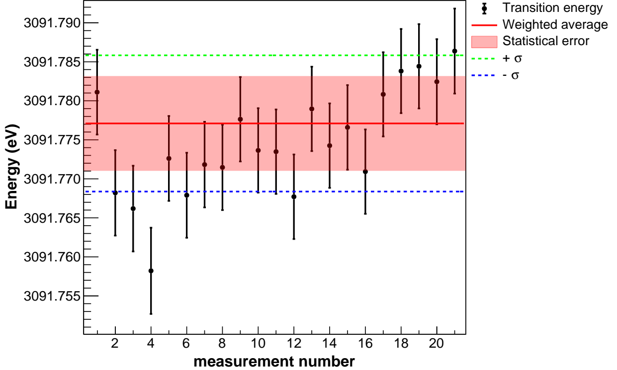
FIG. 11: (Color online) Be-like argon 1s2s^2 2p^1 P_1 \rightarrow 1s^2 2s^2 1 S_0 transition energy values for the different spectra recorded during the experiment. Error bars in each point correspond to the quadratic sum of the peak fitting uncertainty with the uncertainties from Table I, which have random fluctuations only, i.e. , the angle measurement and the temperature correction. The (pink) shaded area correspond to the weighted average of the peak position statistical uncertainty obtained from the fit. The \pm 1\sigma lines combine this statistical uncertainties with all systematic errors from Table I. Every pair of points correspond to one-day data taking (see text for explanations).
