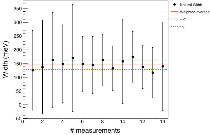
(b) Be-like argon 1s2s^22p^1P_1 \rightarrow 1s^22s^2^1S_0 transition.
