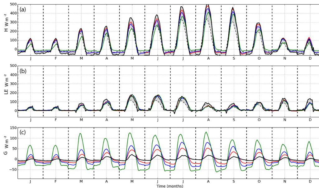
Figure 6. The monthly diurnal cycle composite at Puechabon. MEBL is in red, MEB in blue, ISBA in green, measurements are indicated by a dashed black line and adjusted measurements are represented using a solid black curve. As a visual aid, the area between the latter two curves is shaded. Ideally, model results fall within this area.
